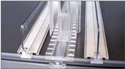
SLIDING RAIL FOR MANUAL PUSHER. Width 42 mm, grey. Length 335 mm | 49092-03/335 Length 435 mm | 49092-03/435
